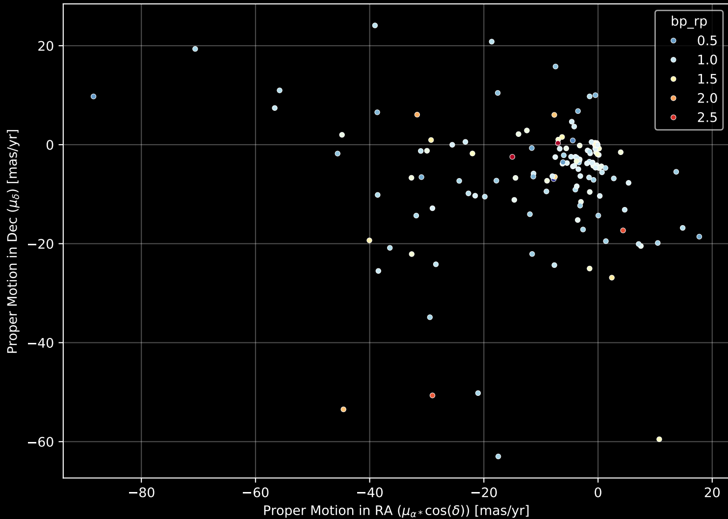
APOGEE DR17 Field: [SEXTANS] Proper Motion Diagram (n= 177)
