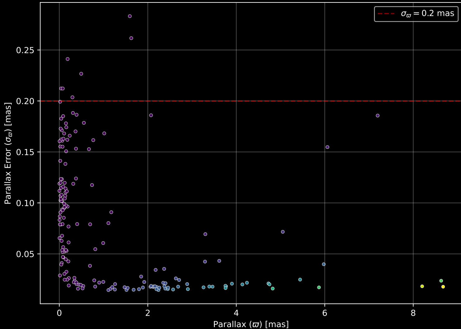
APOGEE DR17 Field: [SEXTANS] Parallax Quality (n= 177)
