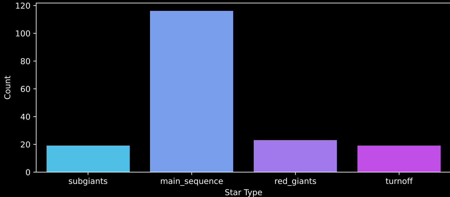
APOGEE DR17 Field: [SEXTANS] Count plot of Star Type
