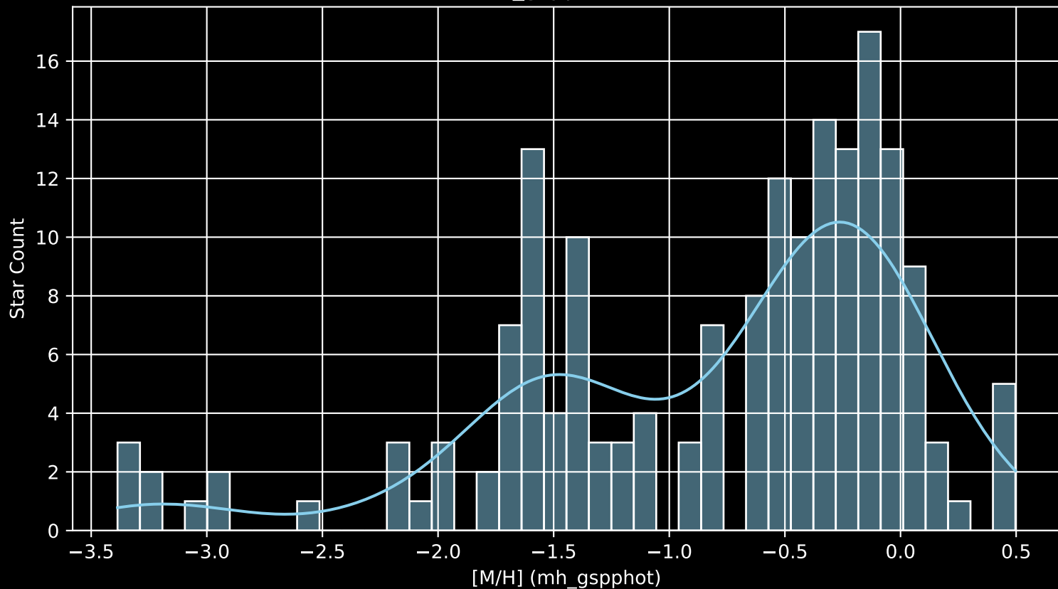
APOGEE DR17 Field: [SEXTANS [M/H] (mh_gspphot) (n= 177)
