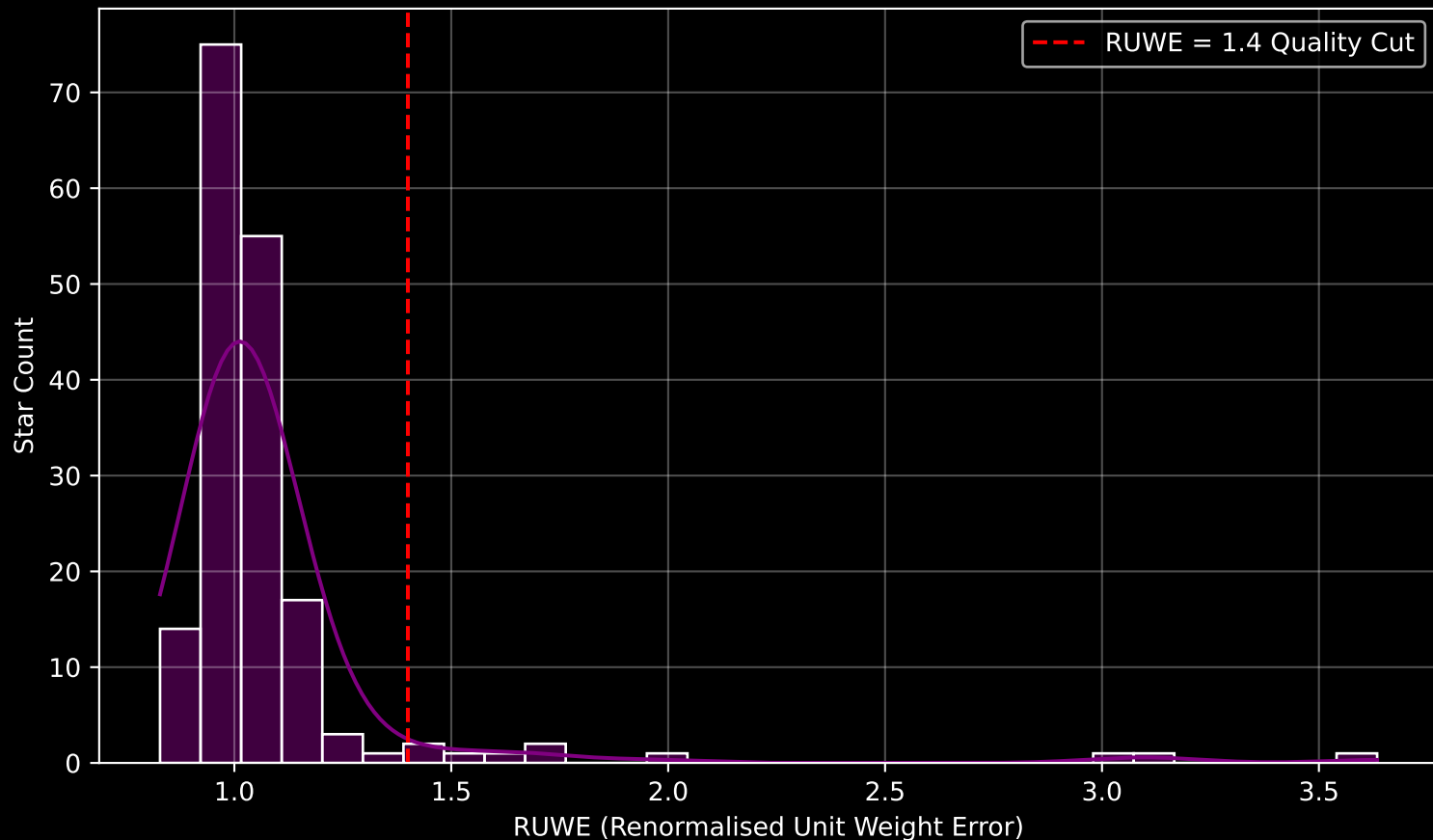
GAPOGEE DR17 Field [SEXTANS] RUWE Distribution (n= 175)
